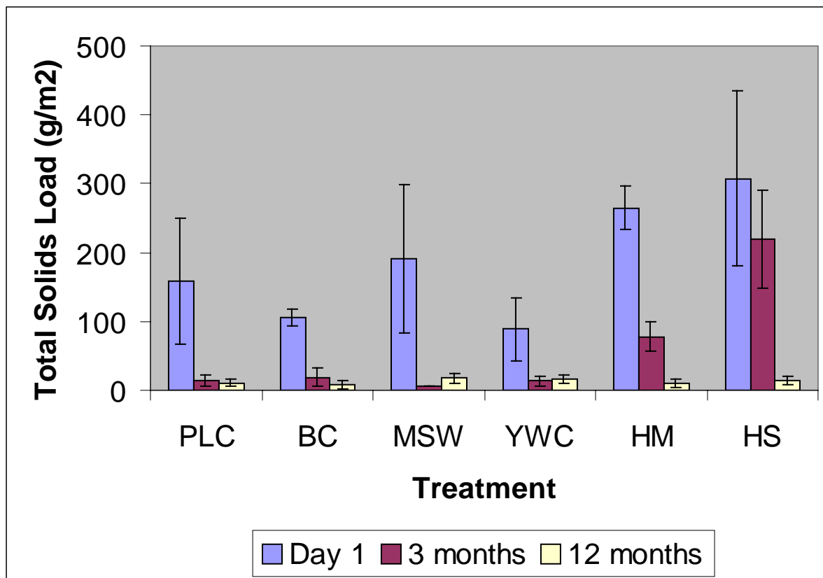
Figure 3.9: Average total solids loads (g/m 2 ) by treatment excluding bare soil control at day one, three months, and twelve months, n = 3.
