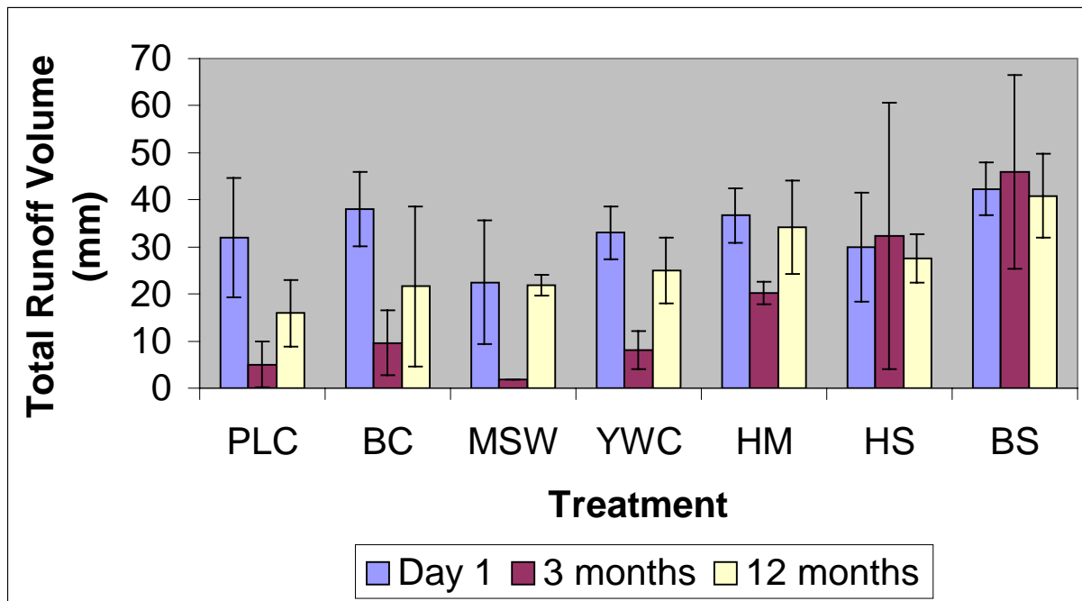
Figure 3.6: Average total runoff volume (mm) by treatment at day one, three months, and twelve months, n = 3 .
