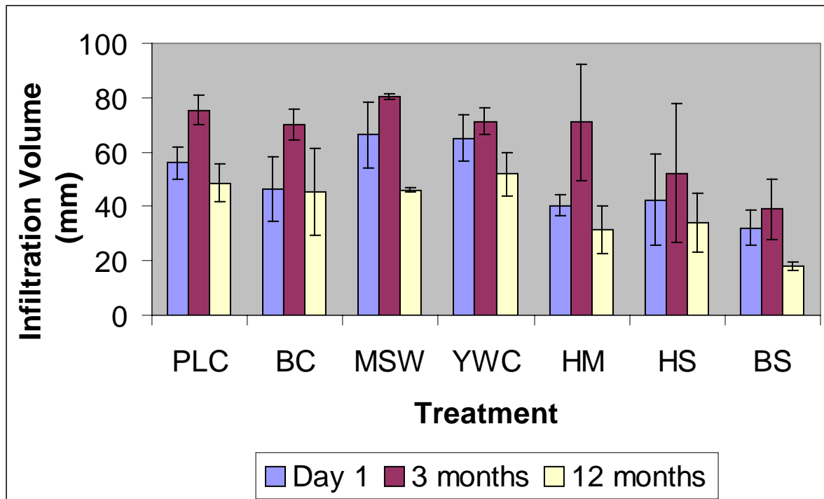
Figure 3.8: Average infiltration volume of rainfall (mm) by treatment at day one, three months and twelve months, n = 3 .
