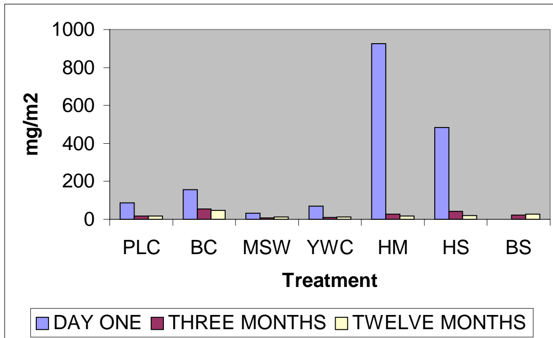
Figure 4.4: Average total P load ( \text{mg}/\text{m}^2 ) in runoff by treatment at day one, three months and twelve months, n = 3 .
