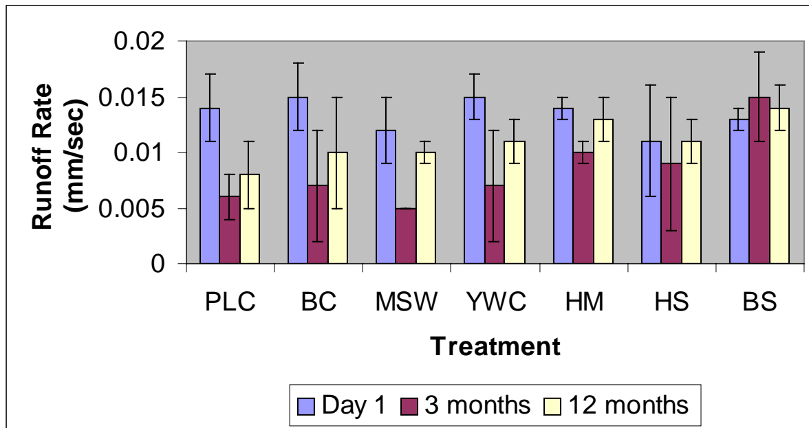
Figure 3.7: Average runoff rate (mm/sec) by treatment at day one, three months and twelve months, n = 3 .
